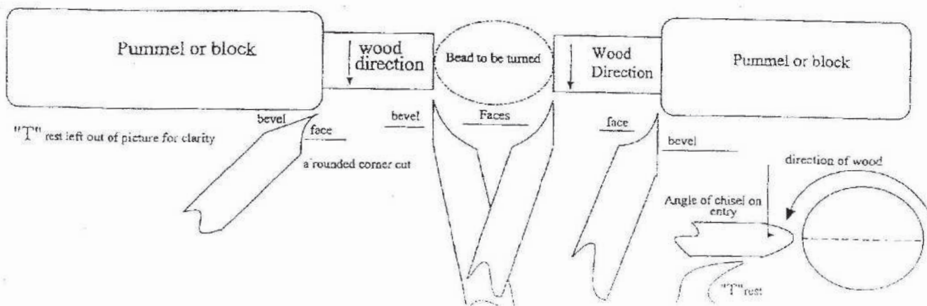
Example of how to chop in with the skewchigouge
