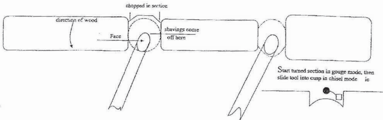
Example 1: Pommel, Bead and shoulder
